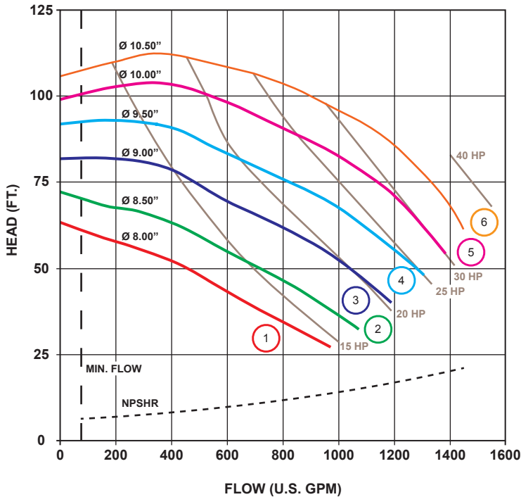
UC6410 (6 x 4 x 10) 1750 RPM, 60Hz
