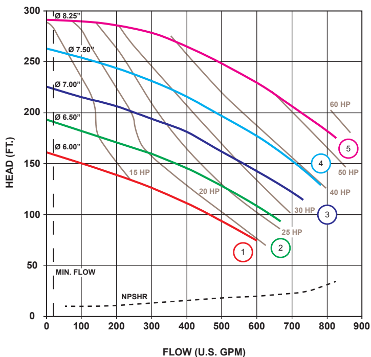
UC438 (4 x 3 x 8) 3500 RPM, 60Hz
