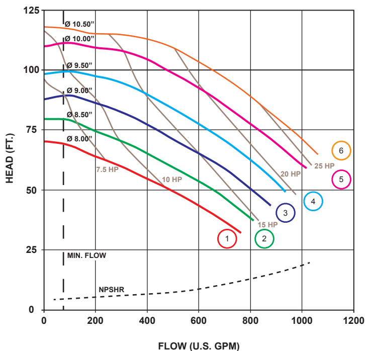
UC4310 (4 x 3 x 10) 1750 RPM, 60Hz
