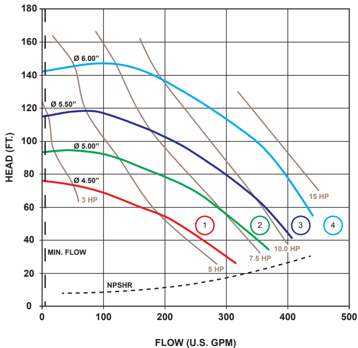
UC326 (3 x 2 x 6) 3500 RPM, 60Hz
