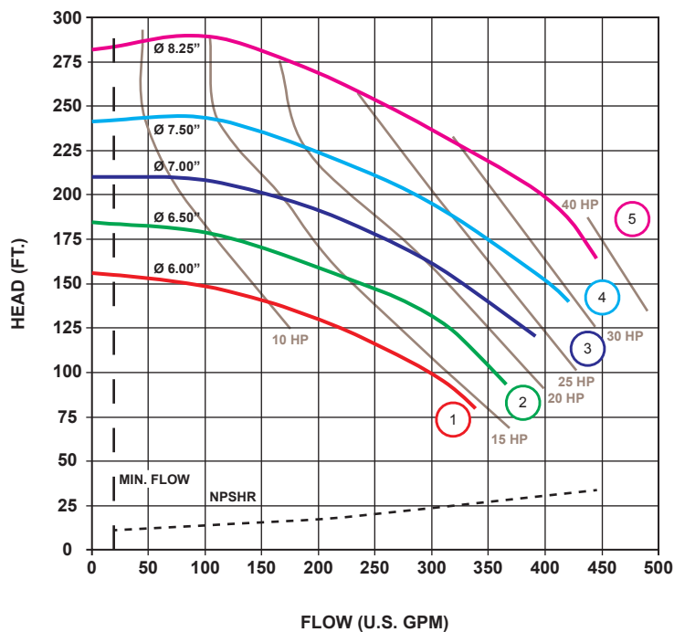
UC328 (3 x 2 x 8) 3500 RPM, 60Hz
