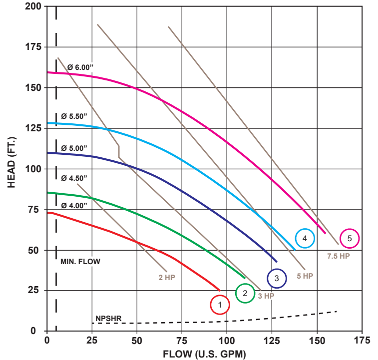
UC1516 3500 RPM, 60Hz
